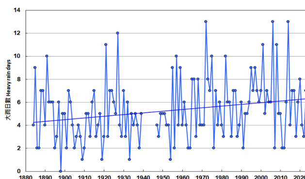
Figure 3.1 Annual number of heavy rainfall days recorded at the Hong Kong Observatory headquarters, 1884–2023
