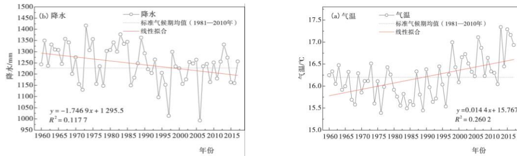
Figure 3.3 Trends in precipitation and temperature in the Chengdu–Chongqing region over the past 50 years [19]
