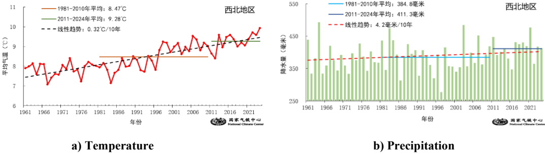
Figure 3.4 Temperature and precipitation changes in Northwestern China, 1961–2024
